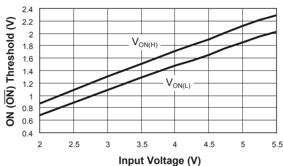
ON ( \overline{ON} ) Threshold vs. Input Voltage
