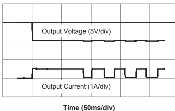
Thermal Shutdown Response
