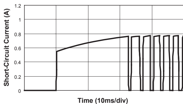
Short-Circuit Current
