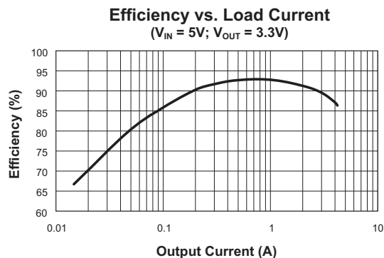
Figure 4: 5V Input, 3.3V Output.
