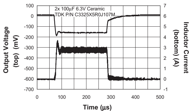
Transient Response
