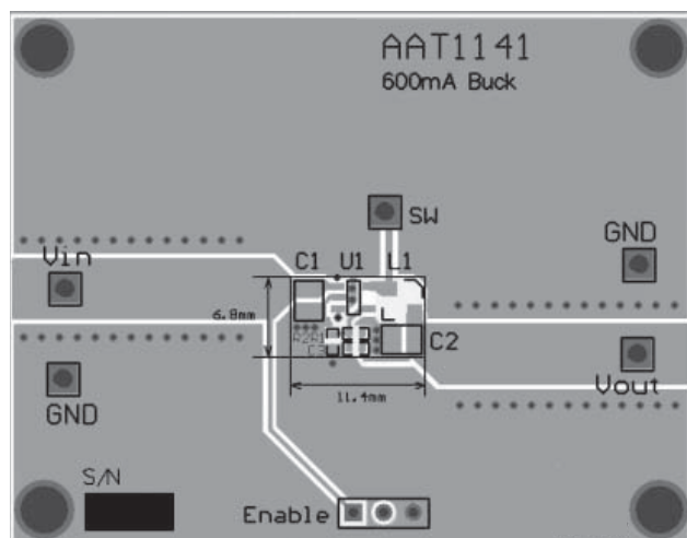
Figure 2: AAT1141 Sample Layout Top Side.
