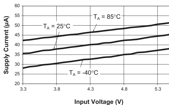
No Load Quiescent Current vs. Input Voltage ( V_{OUT} = 3.0V , L = 6.8\mu H )
