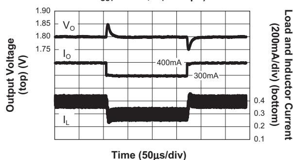
Load Transient Response (300mA to 400mA; V_{IN} = 3.6V ; V_{OUT} = 1.8V ; C_1 = 4.7\mu F )
