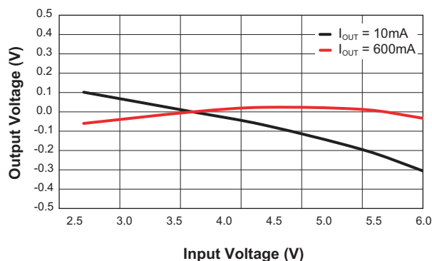
Line Regulation
