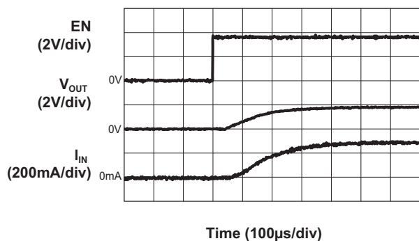
Soft Start
