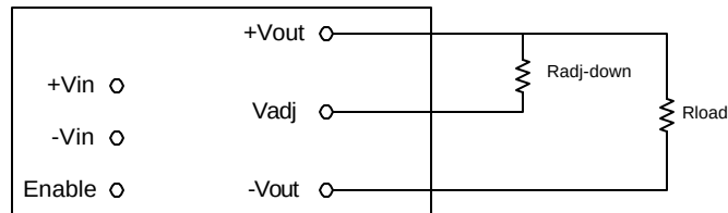
Figure 14 . Circuit Configuration to Decrease Output Voltage.
