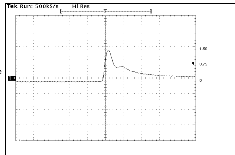
Figure 11. Typical Dynamic Response Step Load Change from 50% to 25% I_{o,max}
