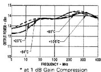
Intercept Point
