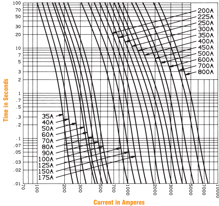
Melting Time – Current Data, 700V Fuses
