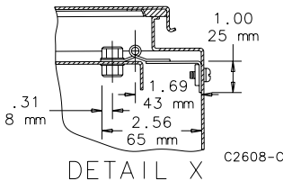
DETAIL X
