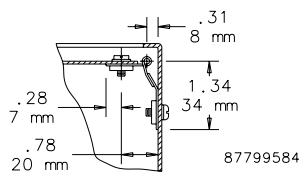
DETAIL X
