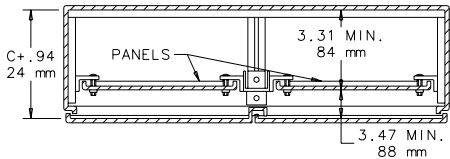
Center Panel Supports Enclosure Section Views
