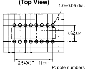
PCB Dimensions (Top View)
