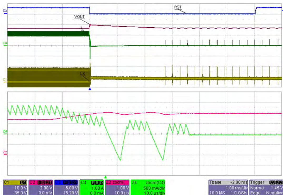
Figure 34. Overvoltage operation
