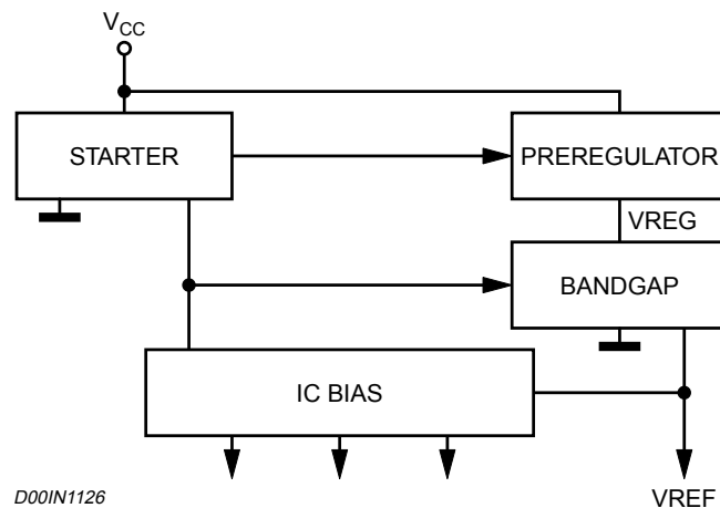
Figure 4. Internal circuit
