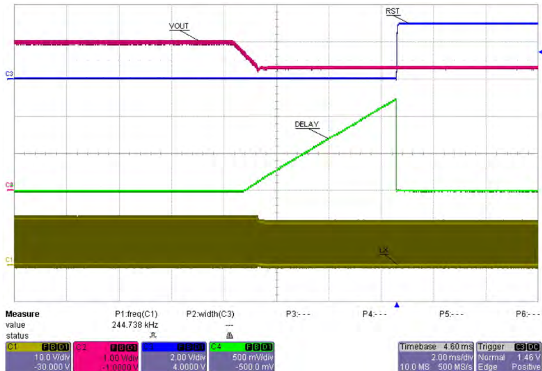
Figure 44. Voltage supervisor operation during OVP
