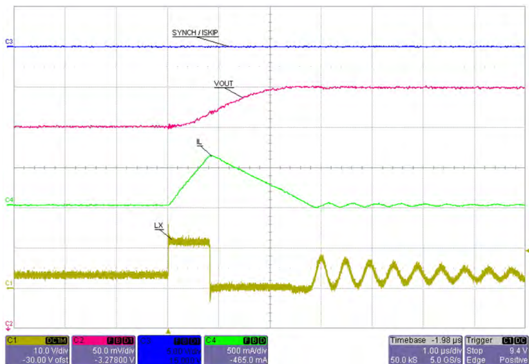
Figure 21. LCM operation with IS_{SKIP_L} = 200\text{ mA} typ. at zero load
