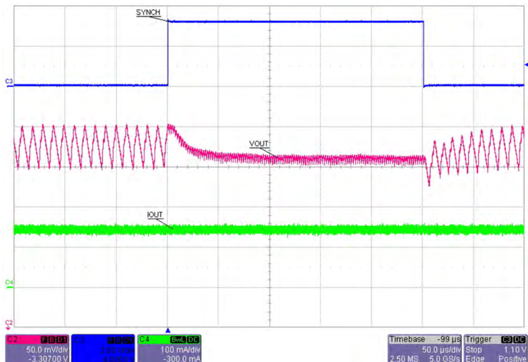
Figure 17. A6986H skip current level transition at I_{LOAD} = 150 mA with L = 10 \mu H
