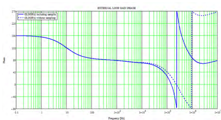
Figure 39. Phase plot
