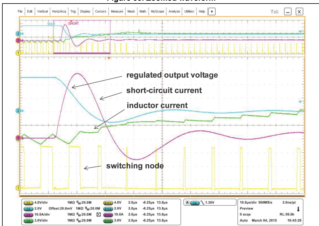
Figure 33. Zoomed waveform
