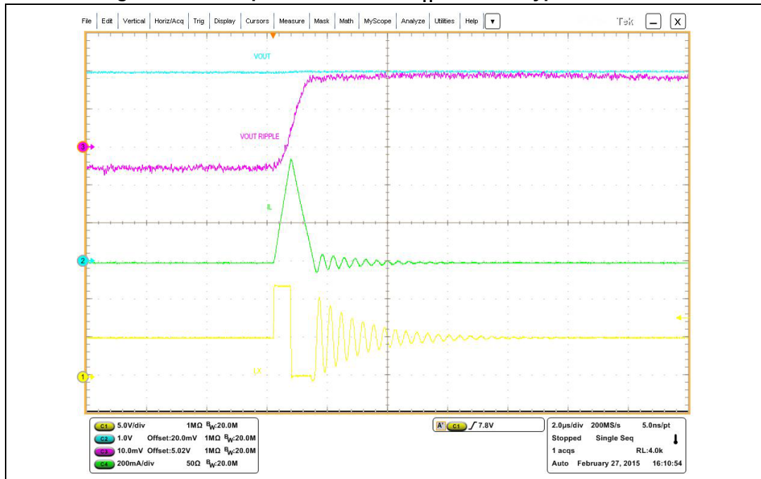
Figure 21. LCM operation with ISKIP_L = 200 mA typ. at zero load
