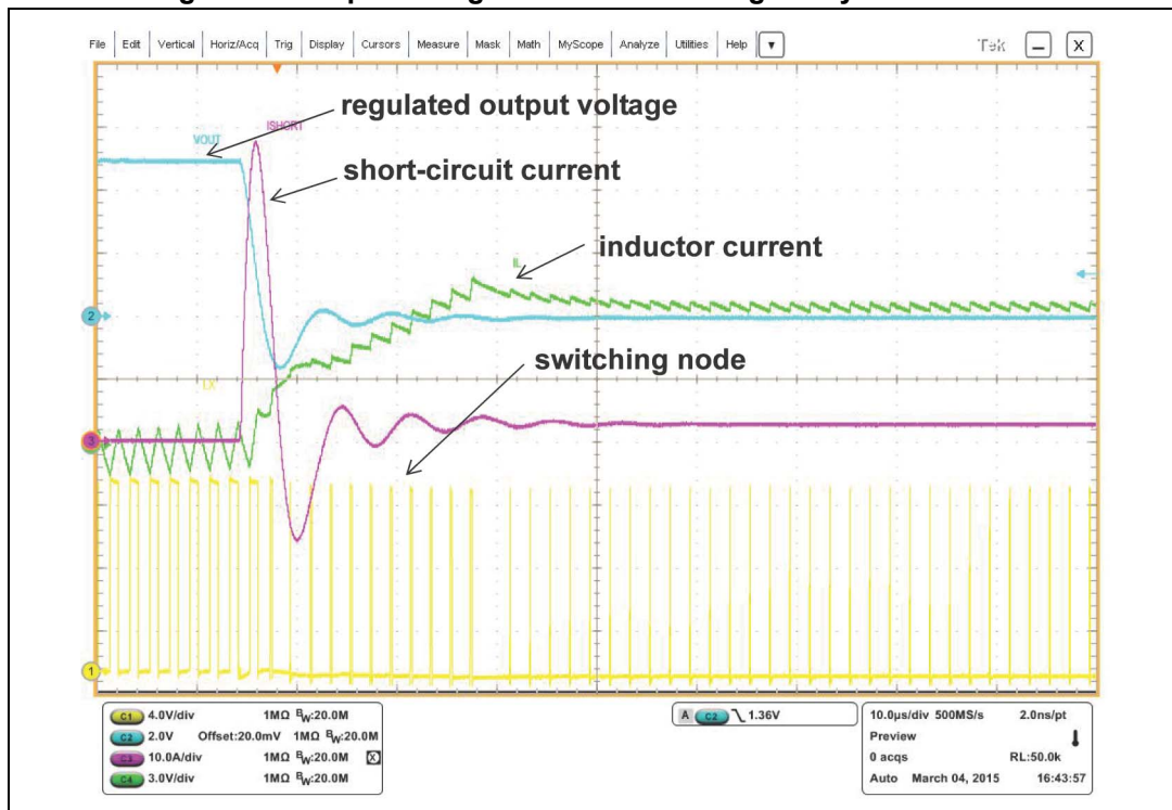
Figure 33. Zoomed waveform
