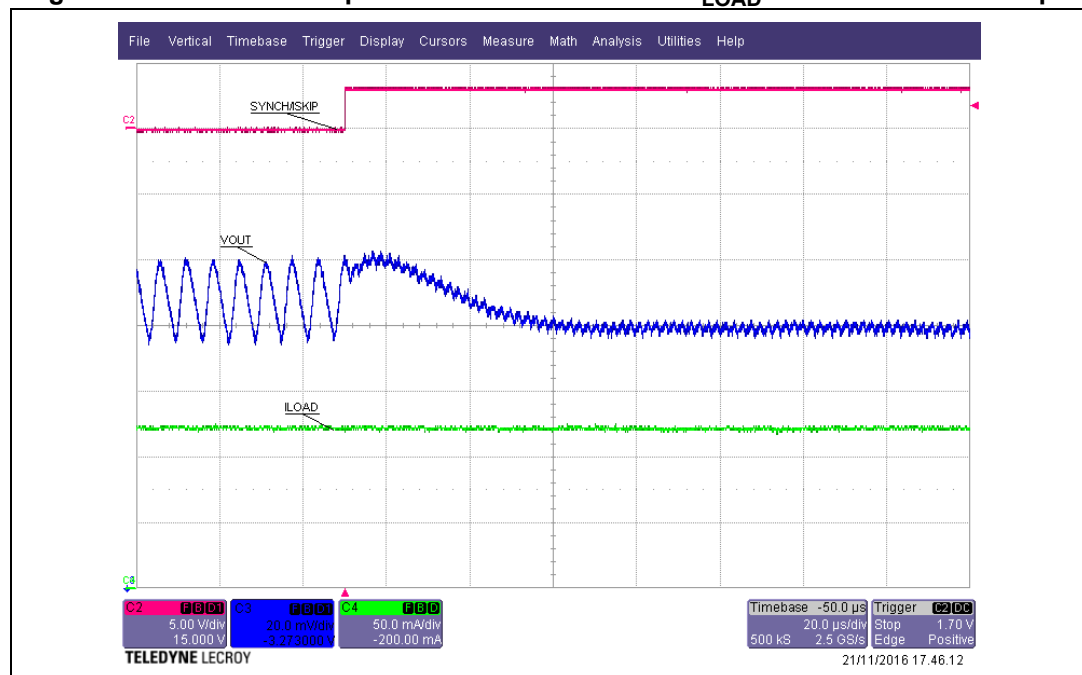
Figure 17. A6986F3V3 skip current level transition at I_{\text{LOAD}} = 125 \text{ mA} with L = 15 \mu\text{H}
