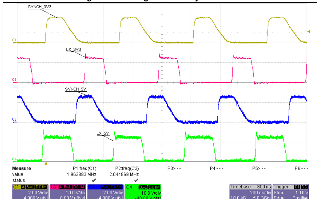
Figure 46. Two regulators not synchronized
