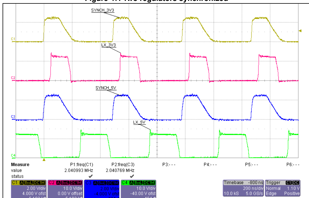
Figure 47. Two regulators synchronized
