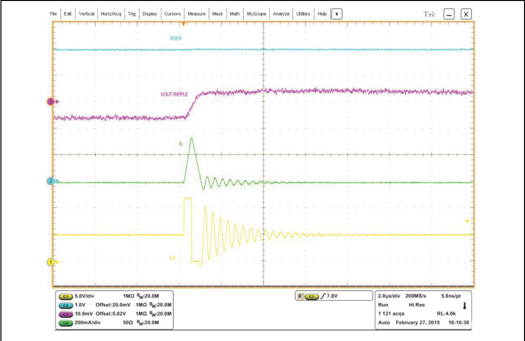
Figure 21. LCM operation with IS_{SKIP_L} = 200\text{ mA typ.} at zero load
