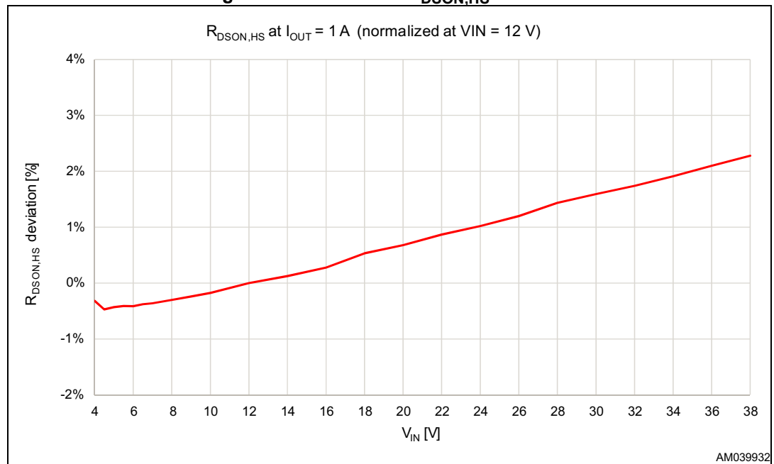
Figure 15. Normalized R_{DS(on),HS} variation
