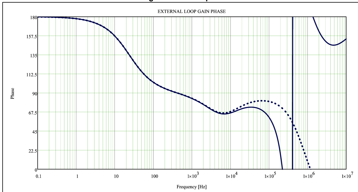
Figure 40. Phase plot
