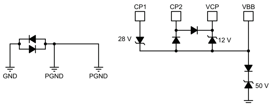
Figure 21a: Supplies and Reference
