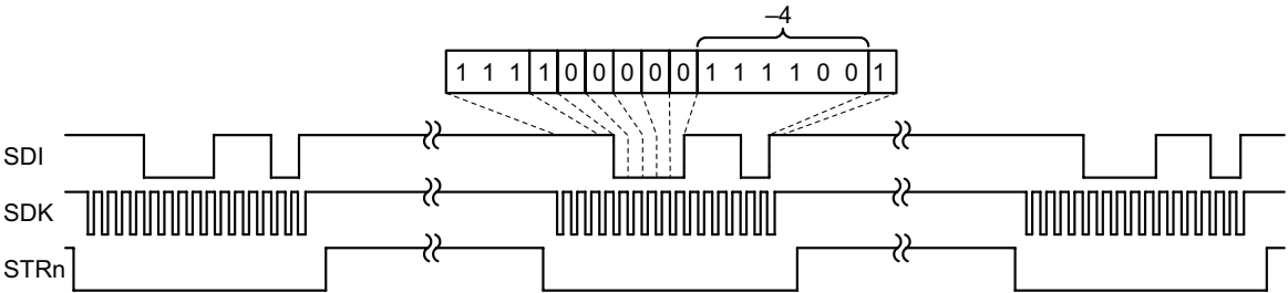
Figure 18: Serial Interface Sequence for Quarter Step in Reverse Direction
