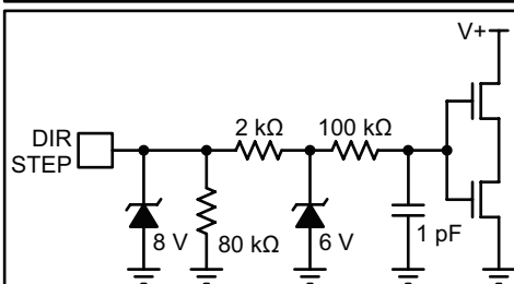
Figure 21f: DIR, STEP Inputs
