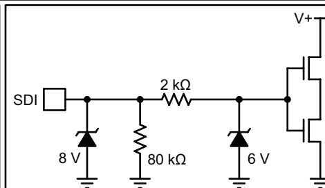
Figure 21d: SDI Input
