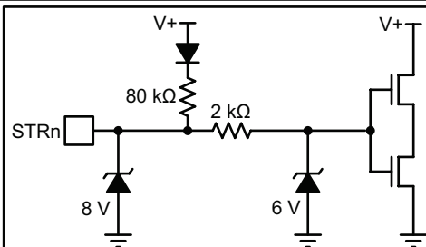
Figure 21c: STRn Input
