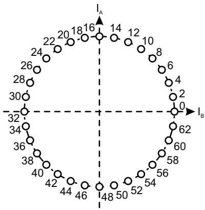
Figure 16: Eighth-Step Phase Diagram
