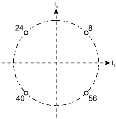
Figure 12: Full-Step 2-Phase Drive Phase Diagram
