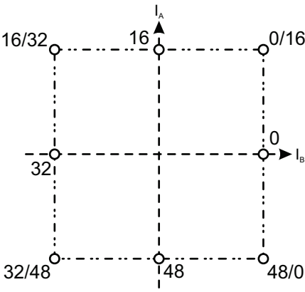
Figure 14: Uncompensated Half-Step Phase Diagram
