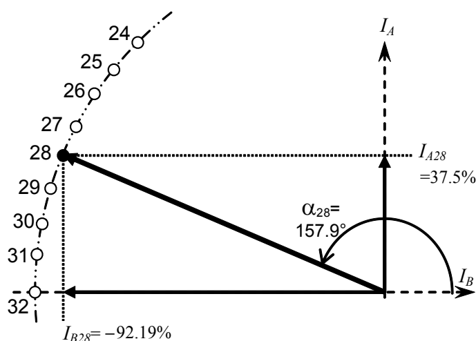
Figure 9: Calculating the Resultant Motor Current
