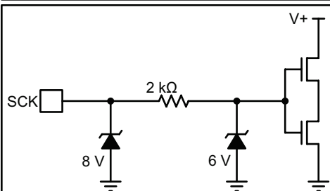
Figure 21b: SCK Input
