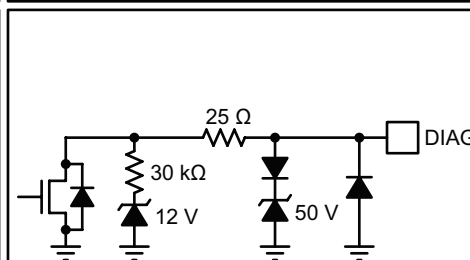
Figure 21g: DIAG Output
