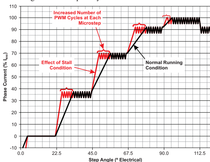
Figure 7: Effect of Stall Condition on Current Rise
