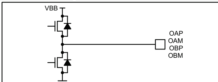
Figure 21i: PHASE Outputs
