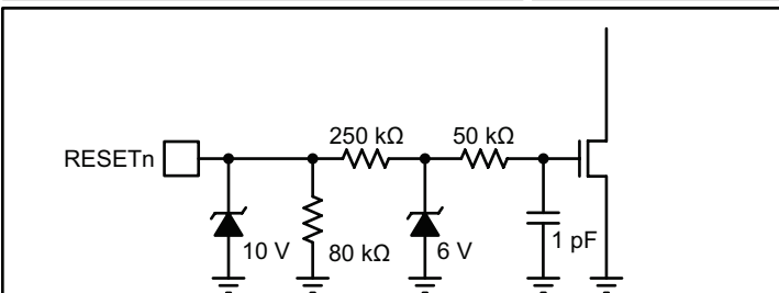
Figure 21h: RESETn Input
