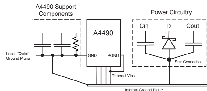
Figure 4. Ground plane configurations
