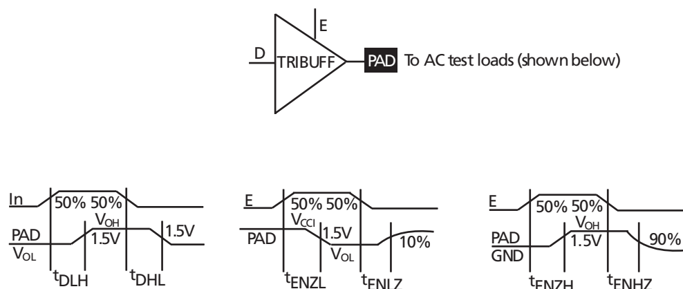
Figure 1-21 • Output Buffer Delays
