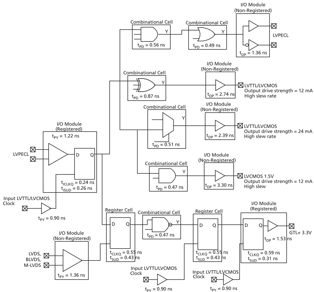
Figure 2-2 • Timing Model
