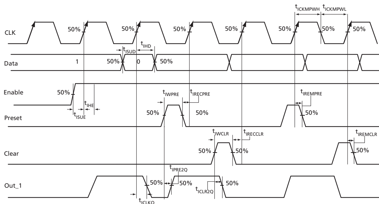
Figure 2-26 • Input Register Timing Diagram
