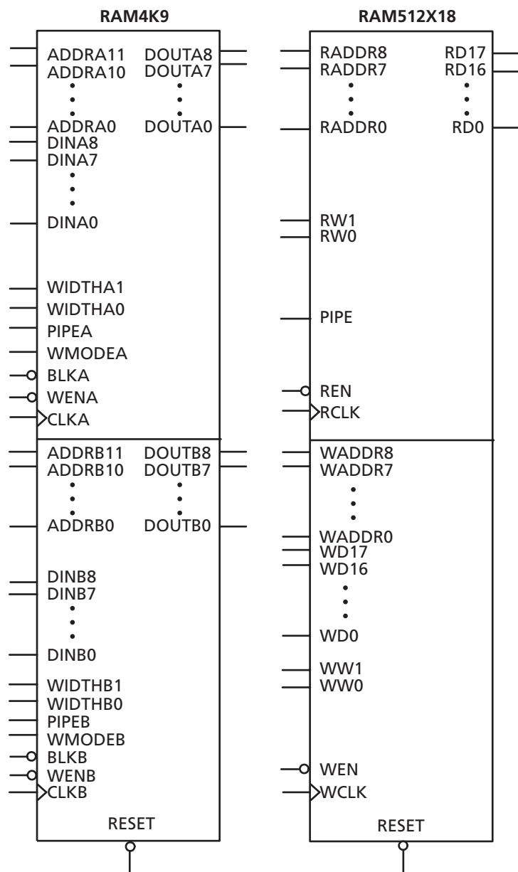
Figure 2-39 • RAM Models
