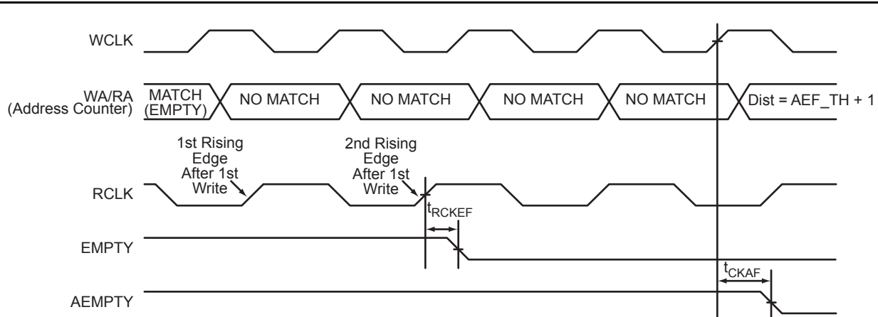
Figure 2-41 • FIFO EMPTY Flag and AEMPTY Flag Deassertion
