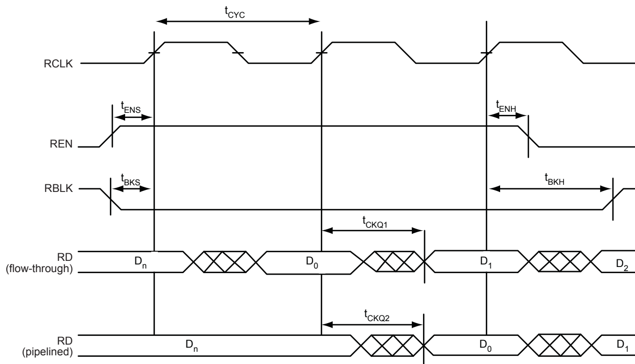
Figure 2-36 • FIFO Read
