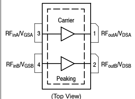
Figure 1. Pin Connections
