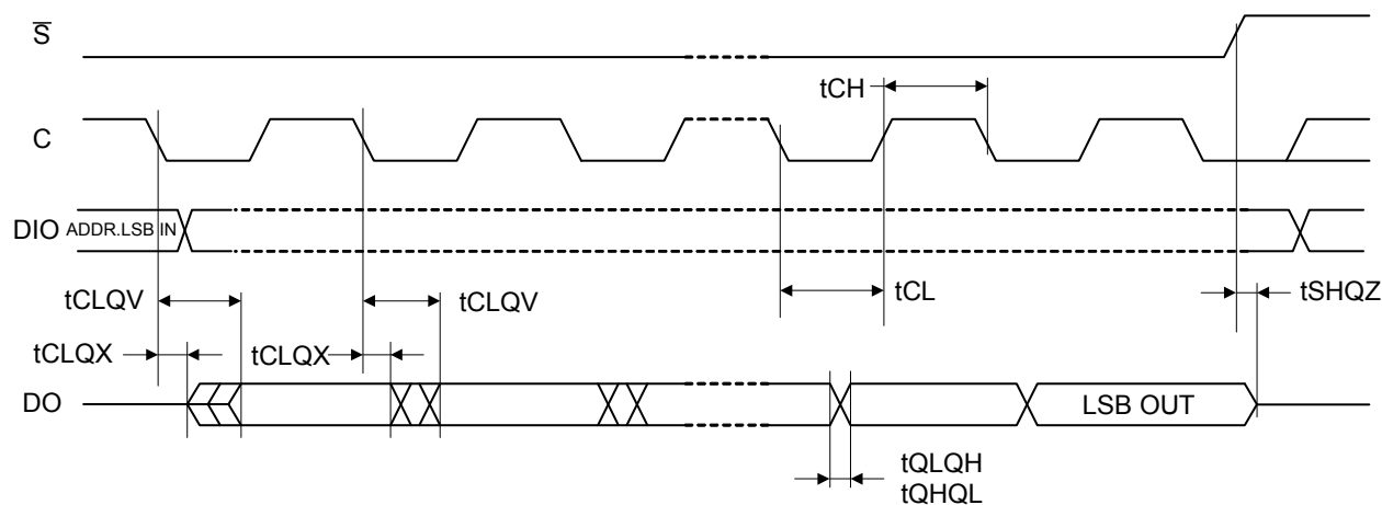
Figure 24. Output Timing
