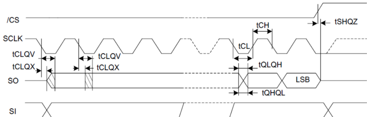
Figure 4. Output Timing
