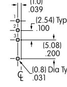
V1 Terminals
