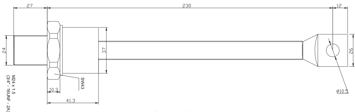
Fig. 15 - Outline Characteristics
