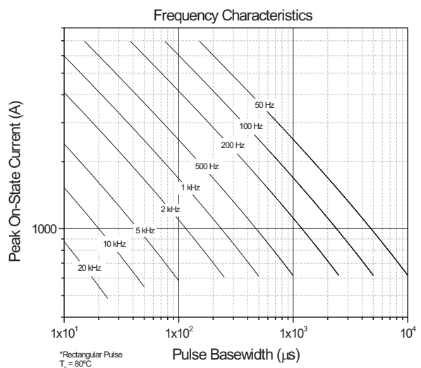
Fig. 10 - Frequency Characteristics
