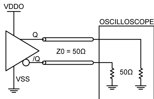
Figure 6. HCSL Output Load and Test Circuit
