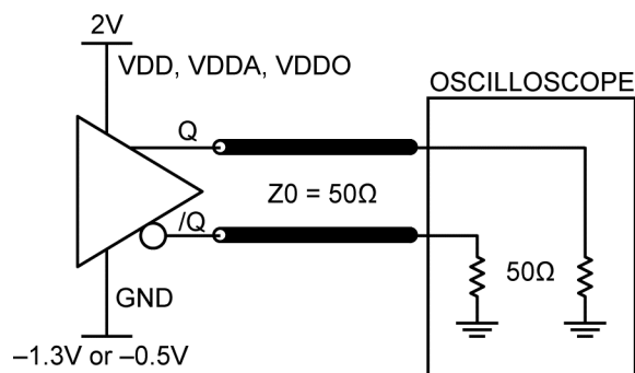
Figure 5. LVPECL Output Load and Test Circuit
