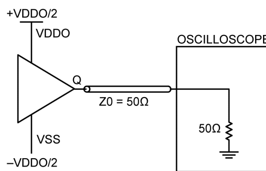
Figure 8. LVCMOS Output Load and Test Circuit
