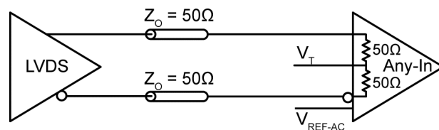
Micrel Any-In Internal Termination
