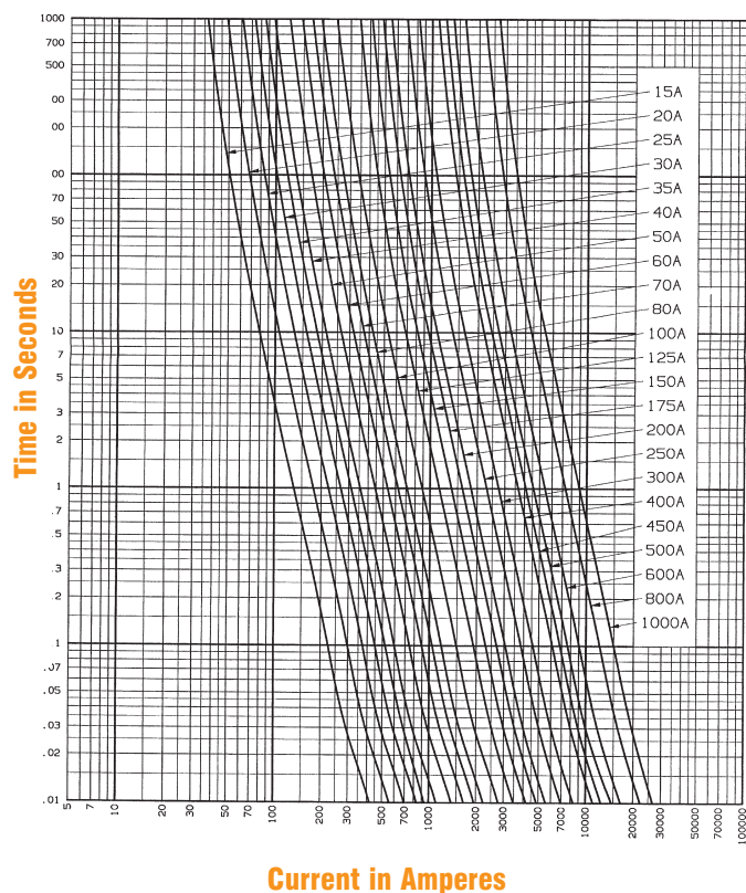
Melting Time – Current Data, 1500V Fuses
