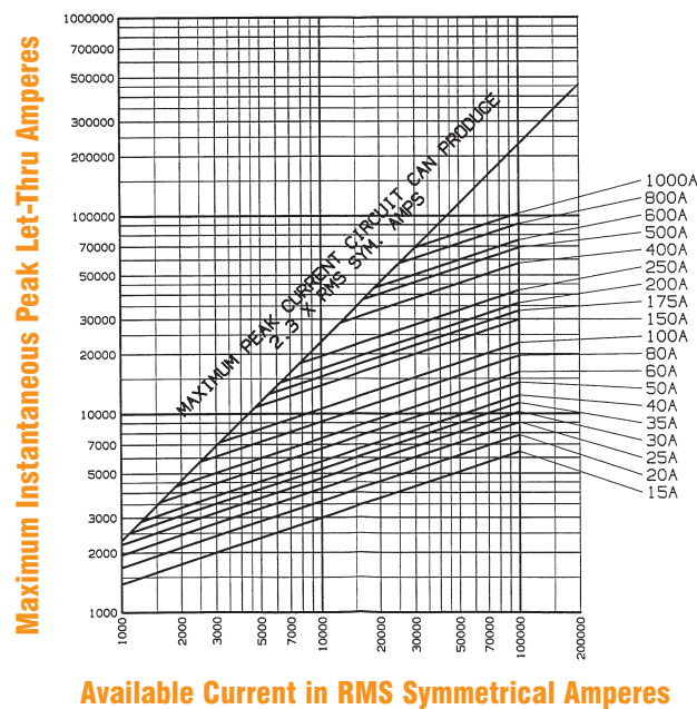
Peak Let-Thru Data – A150X15 to 1000, 1500 VAC
