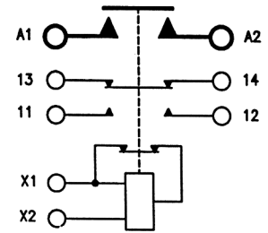
Circuit Configuration 4
