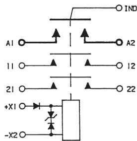
Circuit Configuration 13
