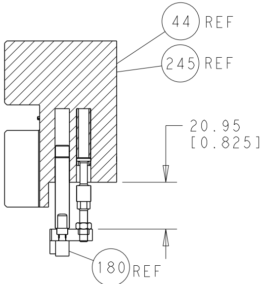
HOLDDOWN SET-UP
