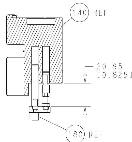
HOLDDOWN SET-UP
