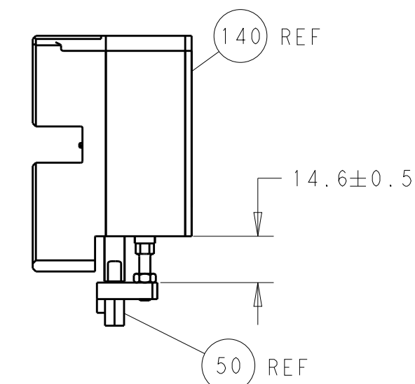
HOLDDOWN SET-UP
