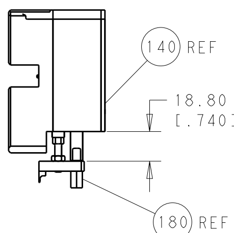
HOLDDOWN SET-UP
