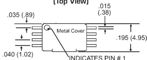
Model 9903 [Top View]
