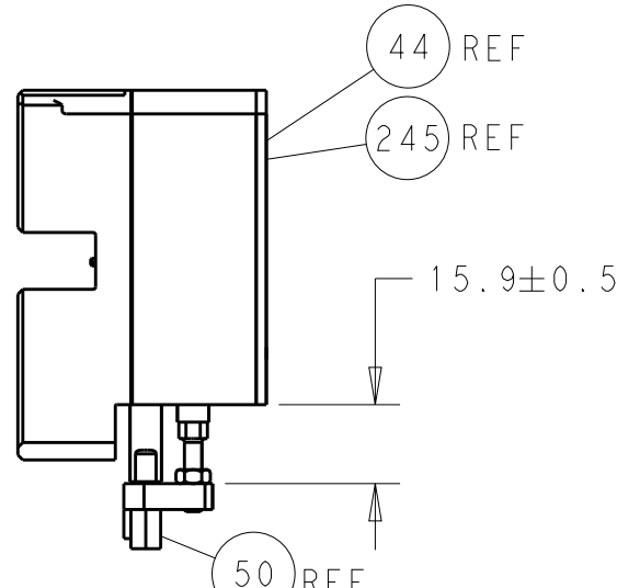
HOLDDOWN SET-UP
