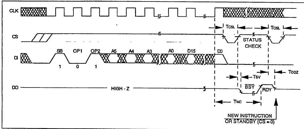
FIGURE 3-2: WRITE MODE
