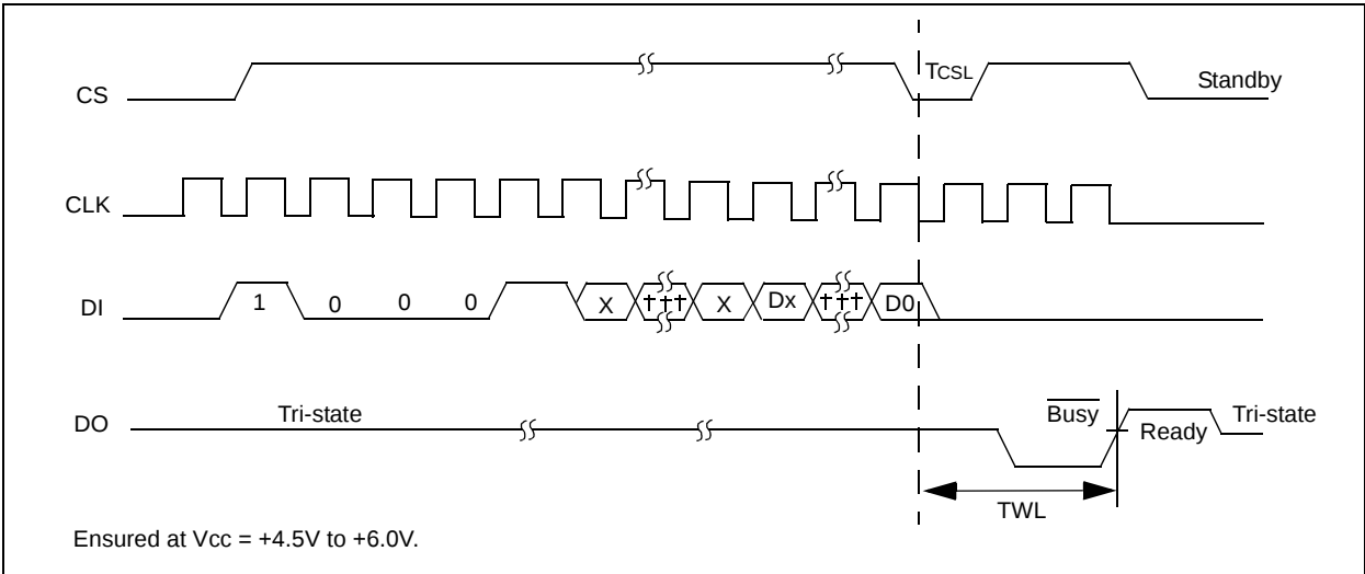
FIGURE 2-6: WRAL TIMING
