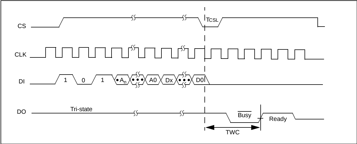
FIGURE 2-5: WRITE TIMING
