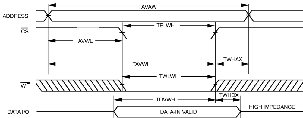
Figure 5. Write Cycle 3. \overline{\text{CS}} Controlled
