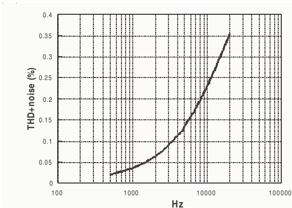
Figure 20. THD + noise vs. frequency (headphone outputs)
