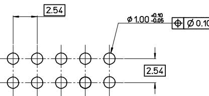
RECOMENDEC P.C. BOARD HOLE PATTERN
