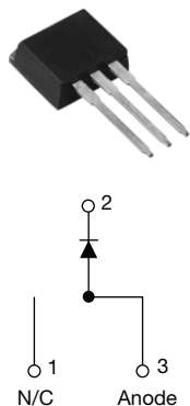
TO-262
