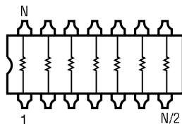
-3 Circuit - Isolated Resistors
