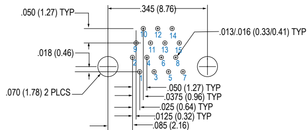
15 Contacts
