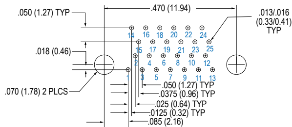
25 Contacts
