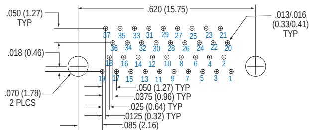
37 Contacts
