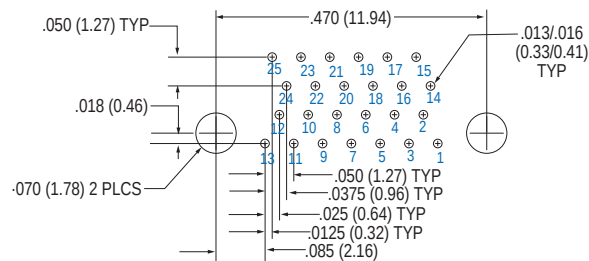
25 Contacts
