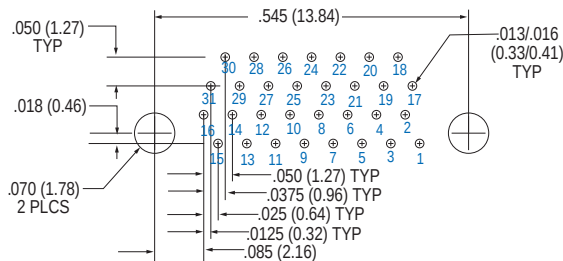
31 Contacts
