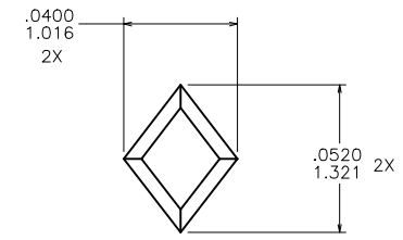
VIEW E-E SCALE 40/1
