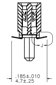
SECTION X-X
