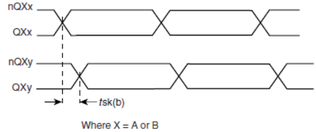
BANK SKEW
