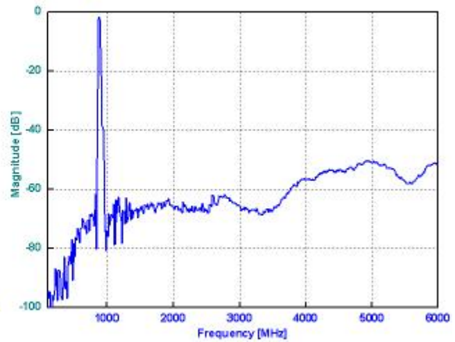
S22
