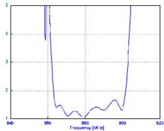
S22
