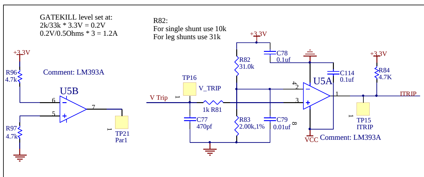
Figure 13 Over current protection circuit on the EVAL-M1-36-45A evaluation board
