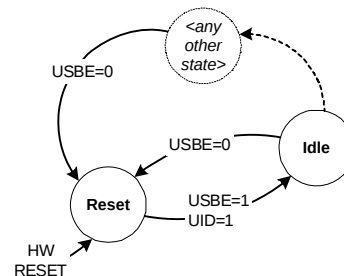
Figure 59. USB Device Controller Reset State Machine
