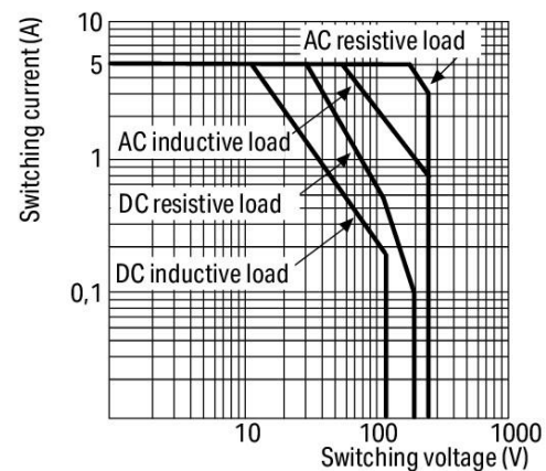
Load limit curve
