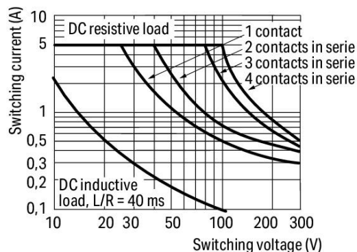
DC load limit curve
