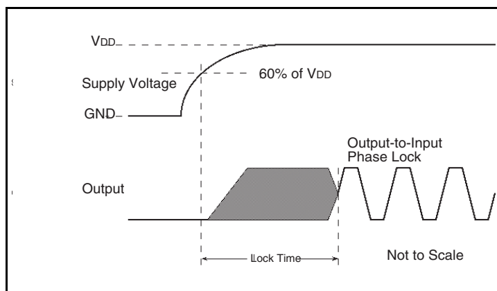
Lock Time
