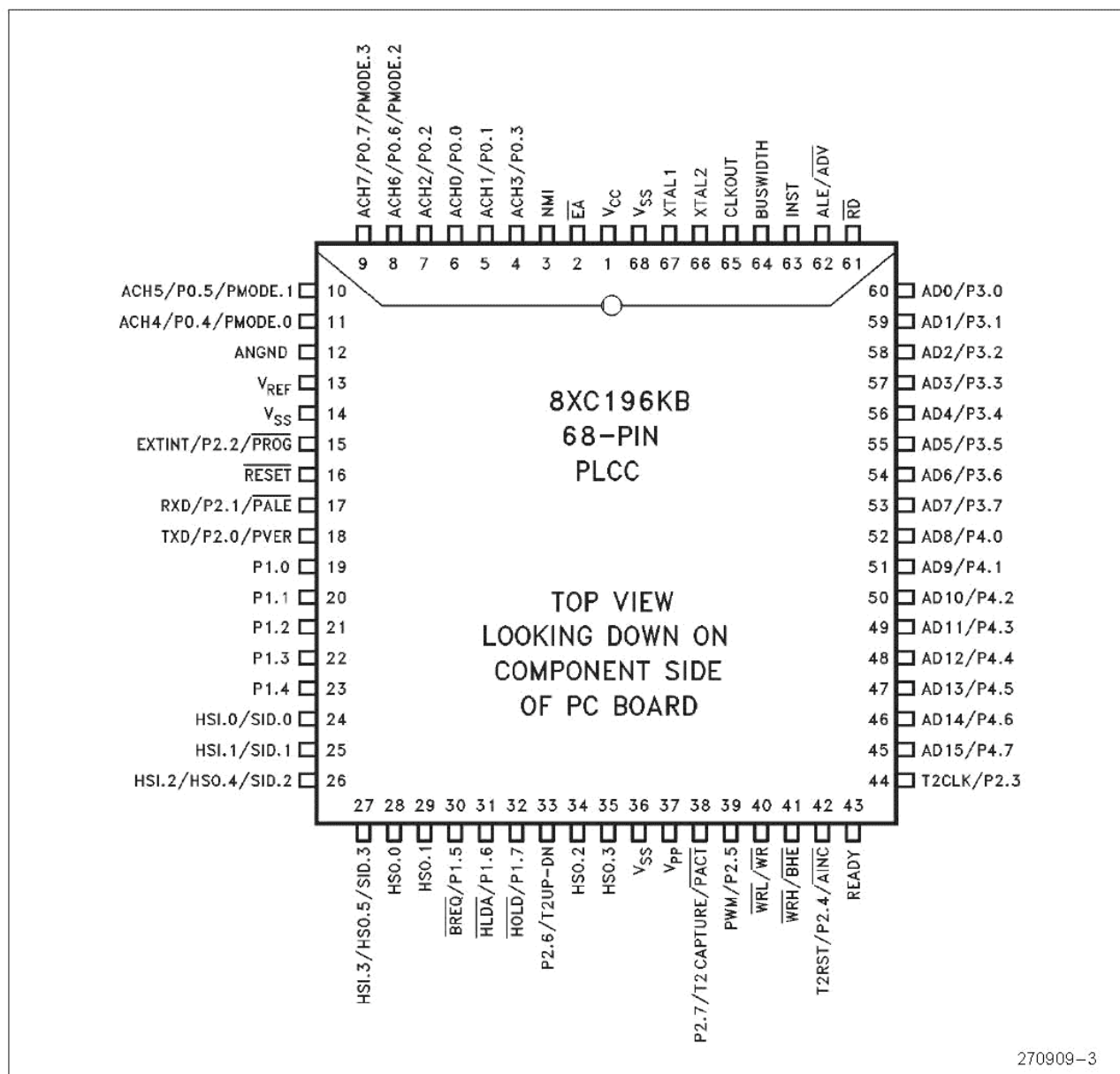
Figure 3. 68-Pin Package (PLCC Top View)
