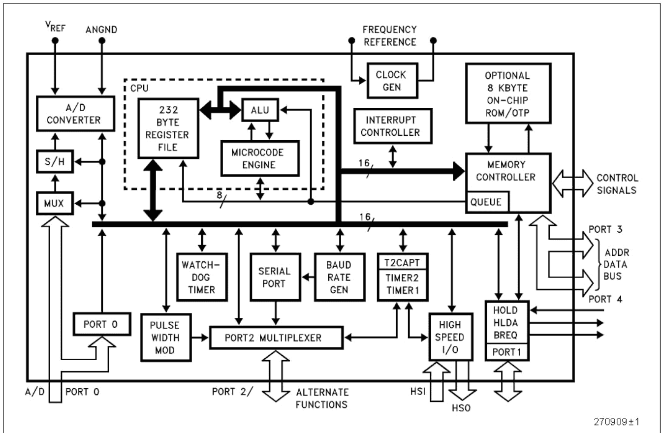
Figure 1. 8XC196KB Block Diagram
