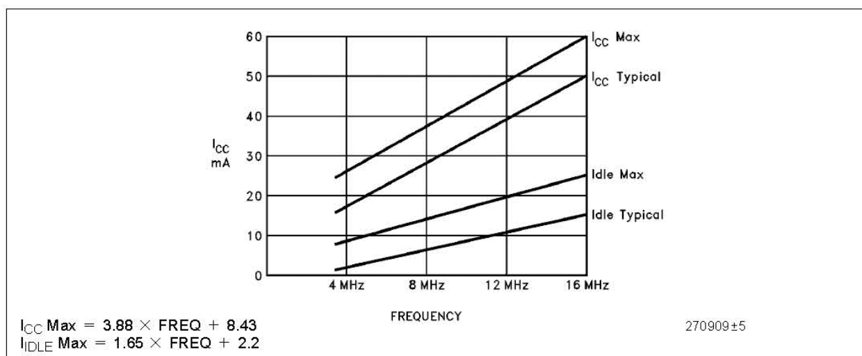
Figure 6. I CC and I IDLE vs Frequency
