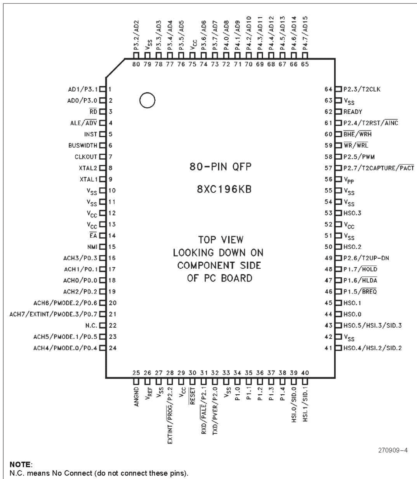
Figure 4. 80-Pin QFP Package
